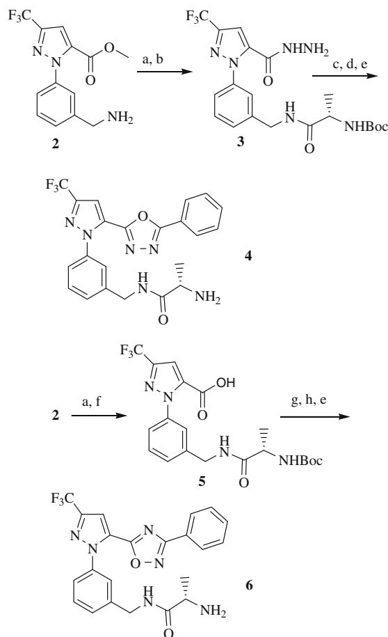
Scheme 1. Reagent and conditions: (a) Boc-L-Ala-OSu, CH 2 Cl 2 , Et 3 N, 92%; (b) hydrazine hydrate, heat, 30 min, 80%; (c) benzoic acid, PyBOP, DIEA, DMF, rt; (d) DIC, DMF, microwave, 150 °C, 20 min, 60% from 3 ; (e) TFA-CH 2 Cl 2 , 92%; (f) 1 N aq NaOH–MeOH, rt, 65%; (g) benamidoxime, CDI, DMF, rt, 4 h; (h) CDI, 100 °C, 4 h, 45% for combined g and h steps.
