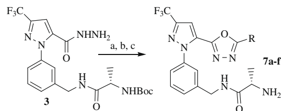
Scheme 2. Reagent and conditions: (a) RCO 2 H, PyBOP, DIEA, DMF, rt or RNCO in case of 7g ; (b) DIC, DMF, microwave, 150 °C, 20 min; (c) TFA-CH 2 Cl 2 , 30–50% from 3 .
