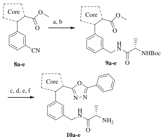
Scheme 3. Reagent and conditions: (a) \text{H}_2 , 10%Pd/C, MeOH, 70–80%; (b) Boc-L-Ala-OSu, \text{CH}_2\text{Cl}_2 , \text{Et}_3\text{N} , 85–95%; (c) hydrazine hydrate, heat, 30 min, 70–80%; (d) benzoic acid, PyBOP, DIEA, DMF, rt; (e) DIC, DMF, microwave, 150 °C, 20 min, 40–60% combined for d and e; (f) TFA- \text{CH}_2\text{Cl}_2 , 80–93%.
