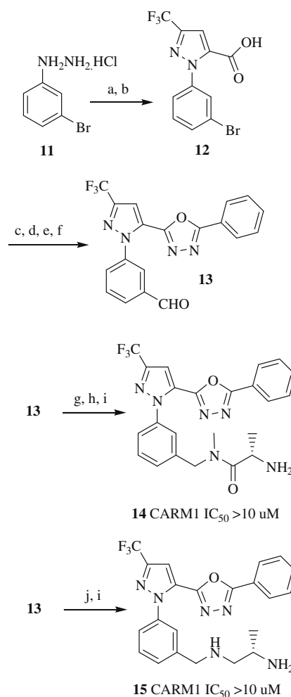
Scheme 4. Reagent and conditions: (a) 4,4,4-trifluoro-1-(furan-2-yl)butane-1,3-dione, AcOH, reflux, 84%; (b) \text{RuCl}_3 , \text{NaIO}_4 , \text{CH}_3\text{CN}-\text{CH}_2\text{Cl}_2-\text{H}_2\text{O} (2:2:3); (c) benzohydrazide, PyBOP, DIPEA, \text{CH}_2\text{Cl}_2 , 59% for combined b and c; (d) DIC, DMF, 150 °C, 60%; (e) tributyl-(vinyl)stannane, \text{Pd}(\text{O})(\text{PPh}_3)_4 , toluene, 110 °C, 65%; (f) \text{HCOOH} , \text{H}_2\text{O}_2 , \text{HIO}_4 , 73%; (g) methylamine HCl, \text{Ti}(\text{OiPr})_4 , \text{NaBH}_4 , EtOH, 50%; (h) Boc-Ala-OH, EDC-HCl, HOBT, DIPEA, DMF, 91%; (i) HCl-dioxane, 49–60%; (j) Boc-alaninal, \text{NaH B}(\text{OAc})_3 , THF, 60%.
